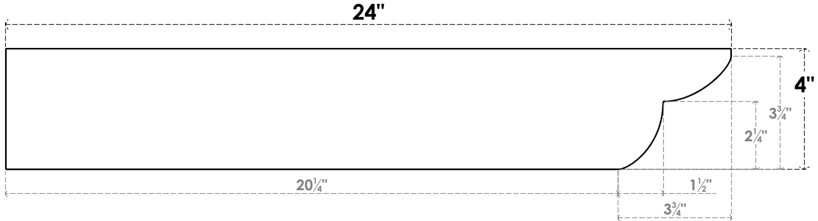
SIDE PROFILE
